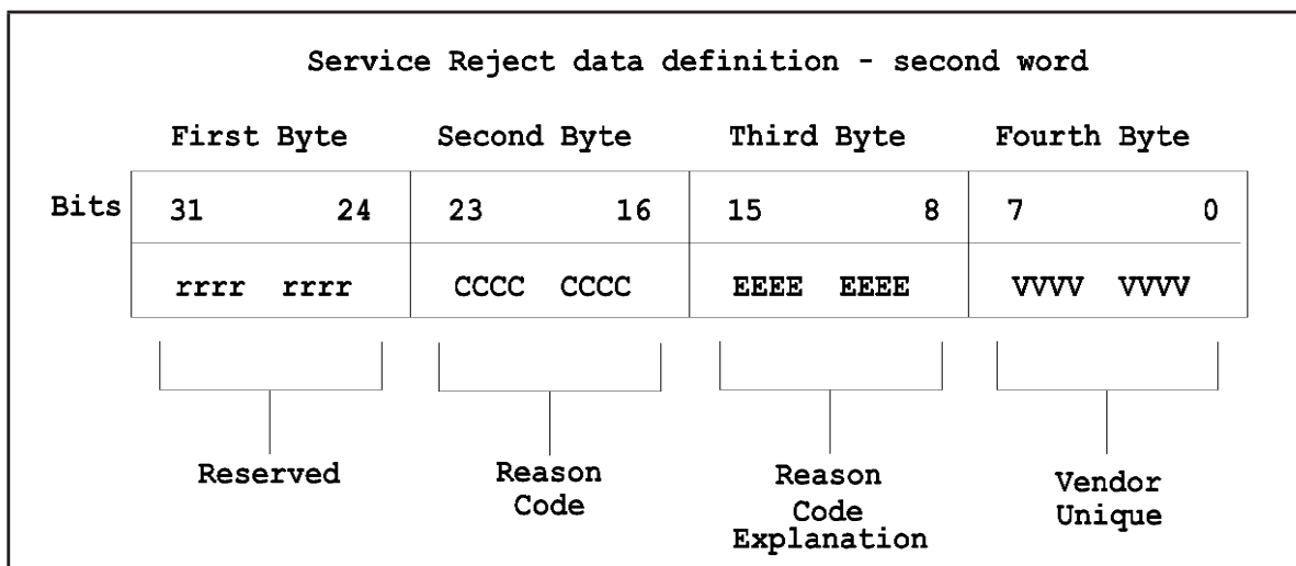
Figure 3 – LS_RJT format
