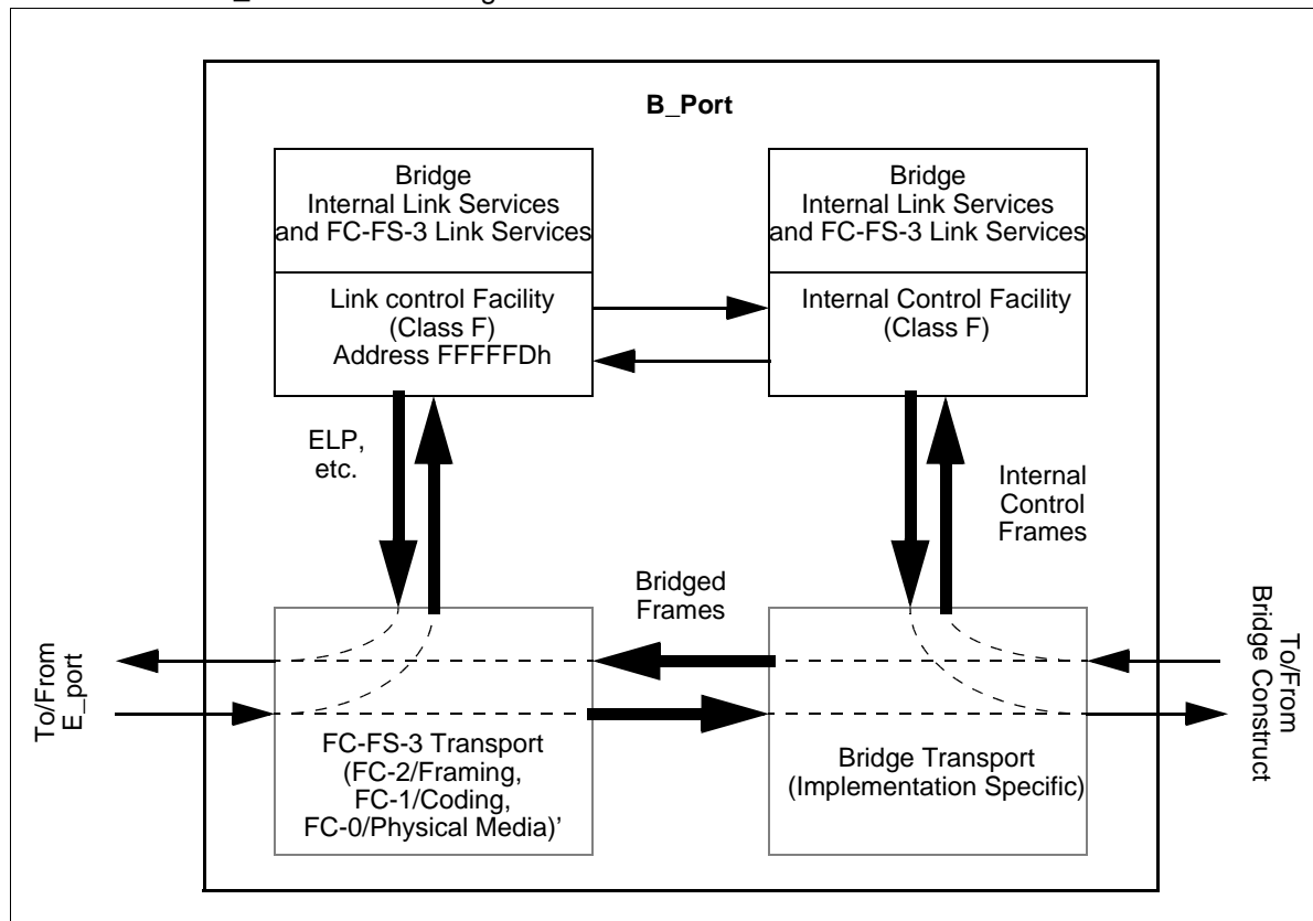
Figure 9 – B_Port Model
