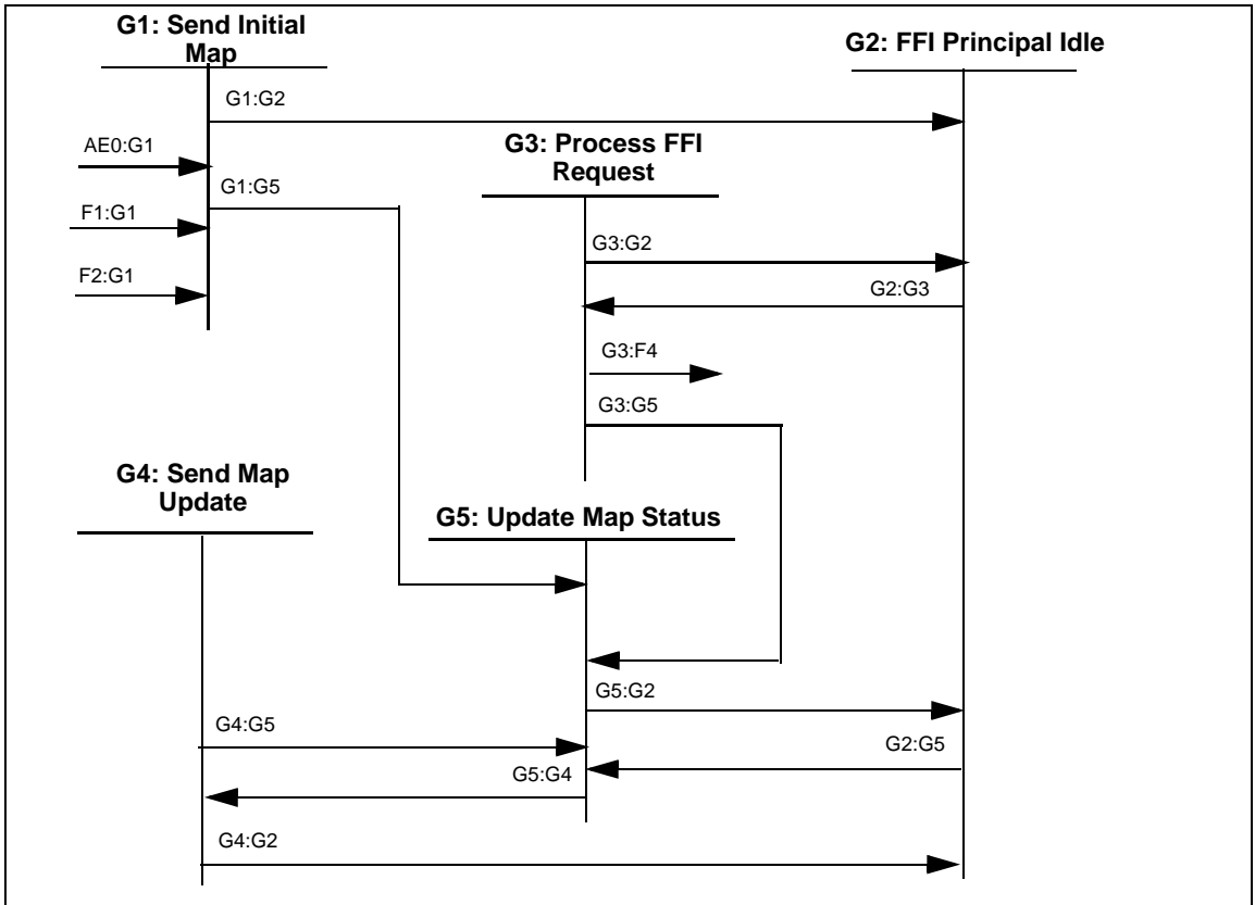
Figure D.3 – FFI Domain Topology Map Distribution State Machine, AE Principal Switch
