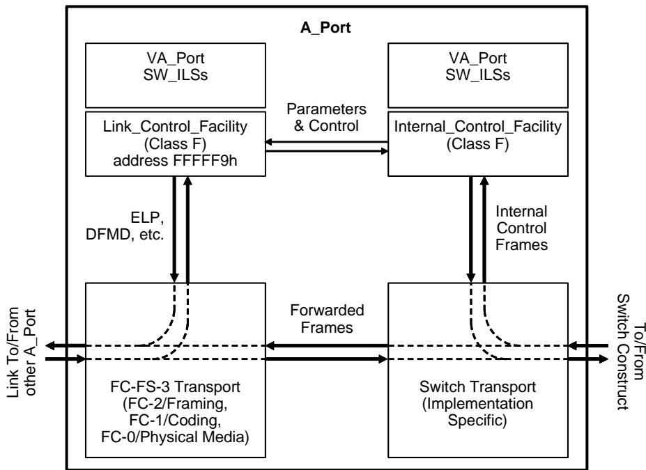
Figure 48 – A_Port Model
