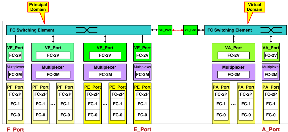
Figure 45 – Controlling Switch Functional Model
