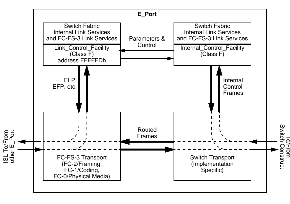
Figure 8 – E_Port Model
