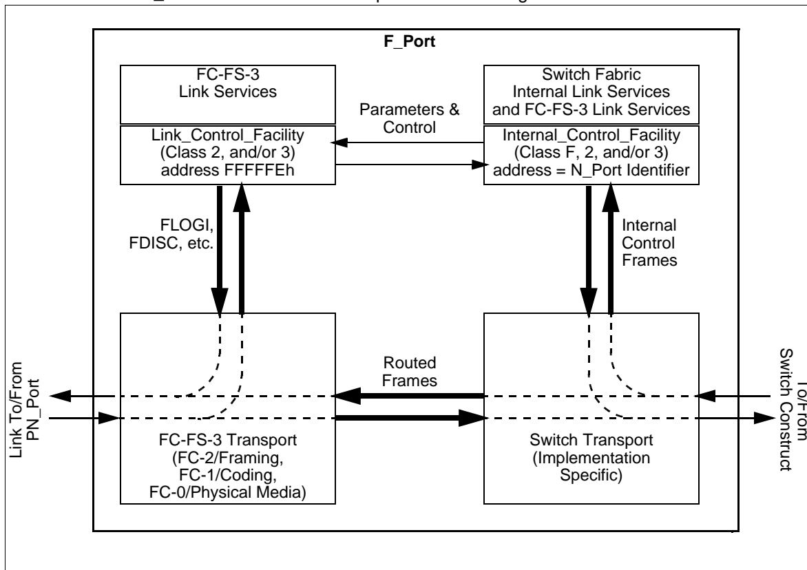
Figure 6 – F_Port Model
