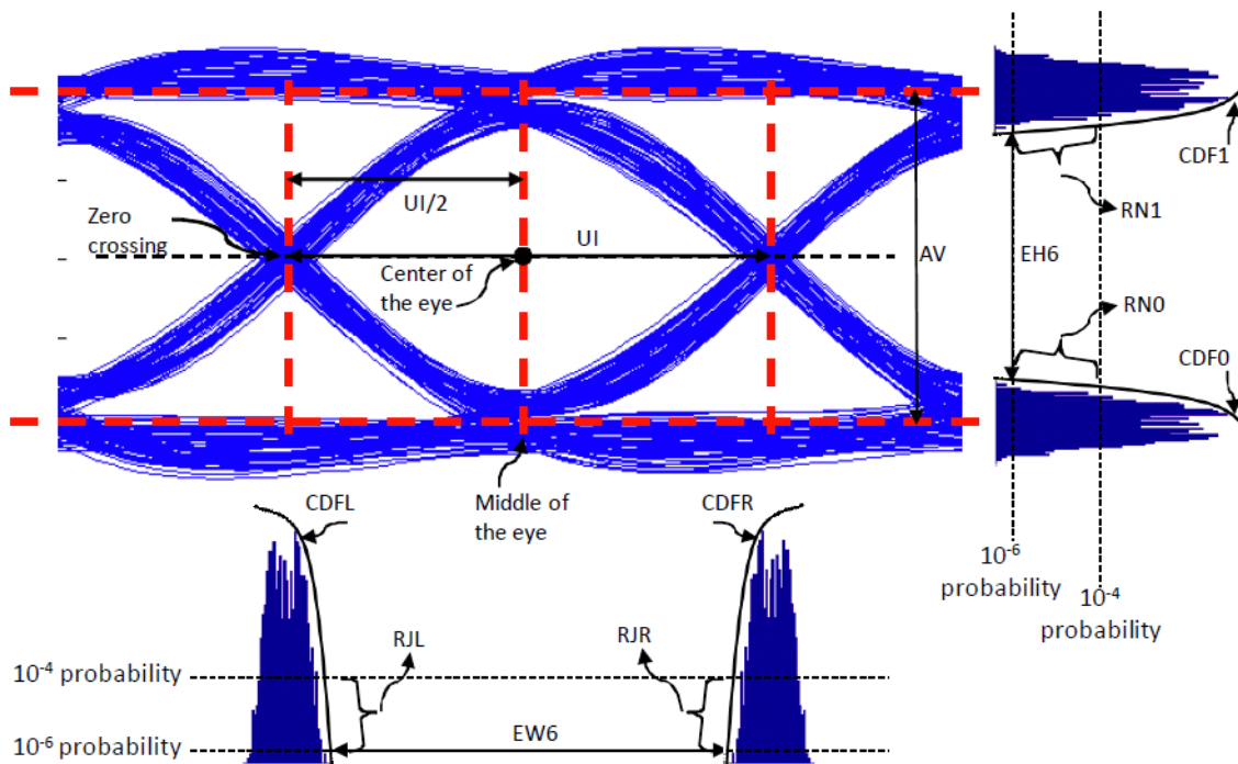
Figure 3.11 - Compliance test point B and C jitter and eye height measurement
