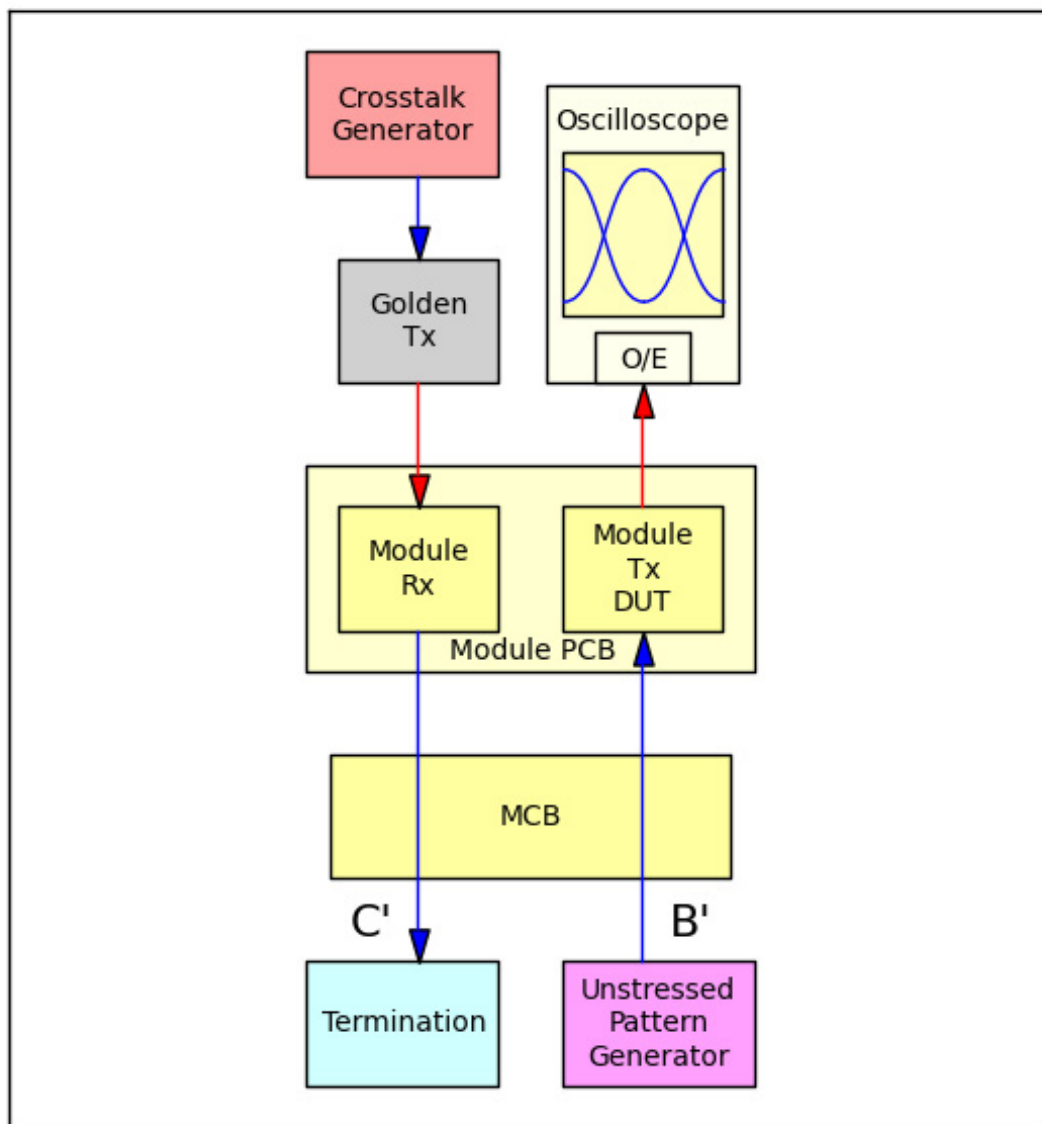
Figure 3.5 - Module optical output compliance test configuration
