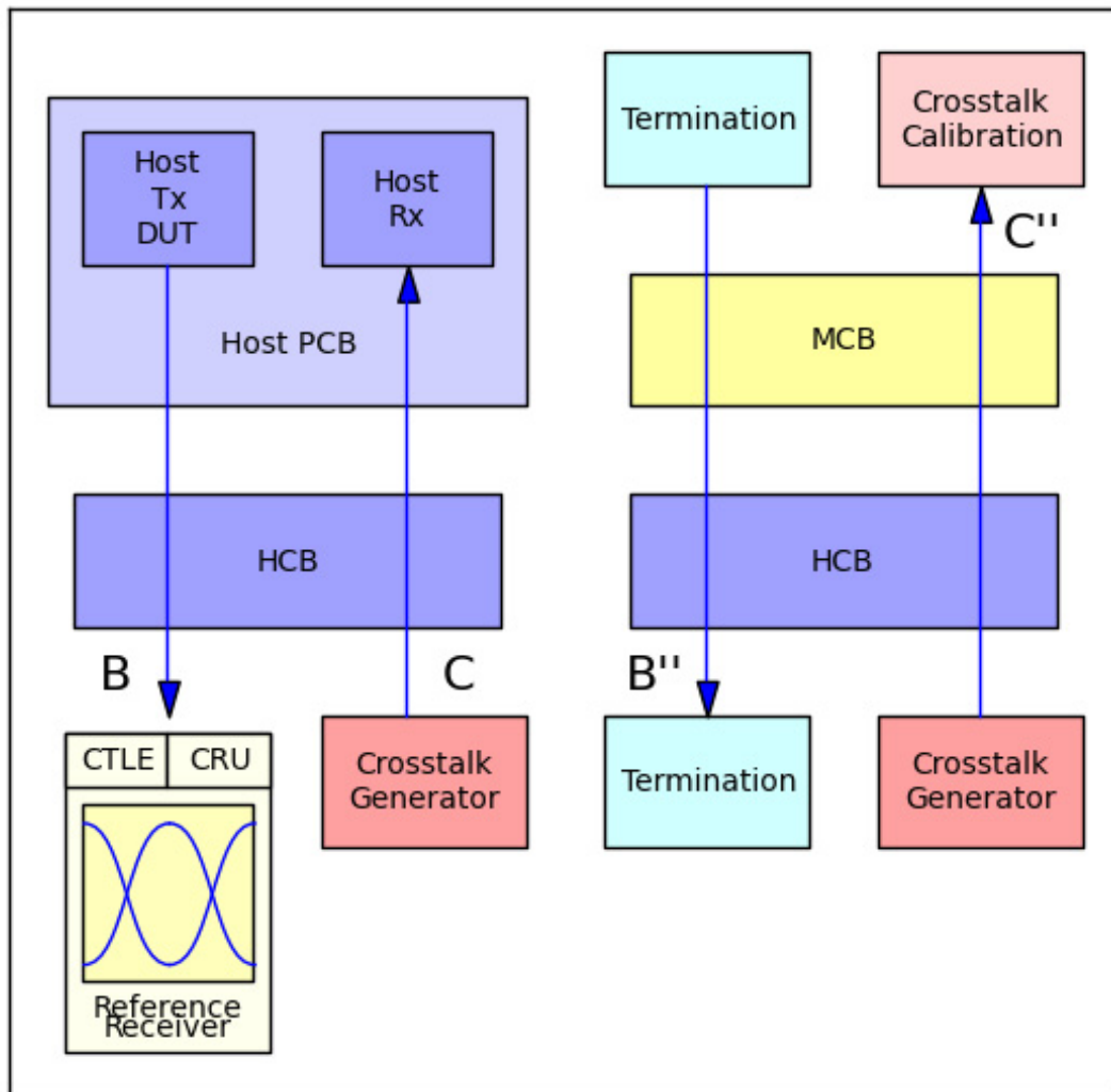
Figure 3.1 - Host output compliance test configuration (left) and crosstalk calibration (right)
