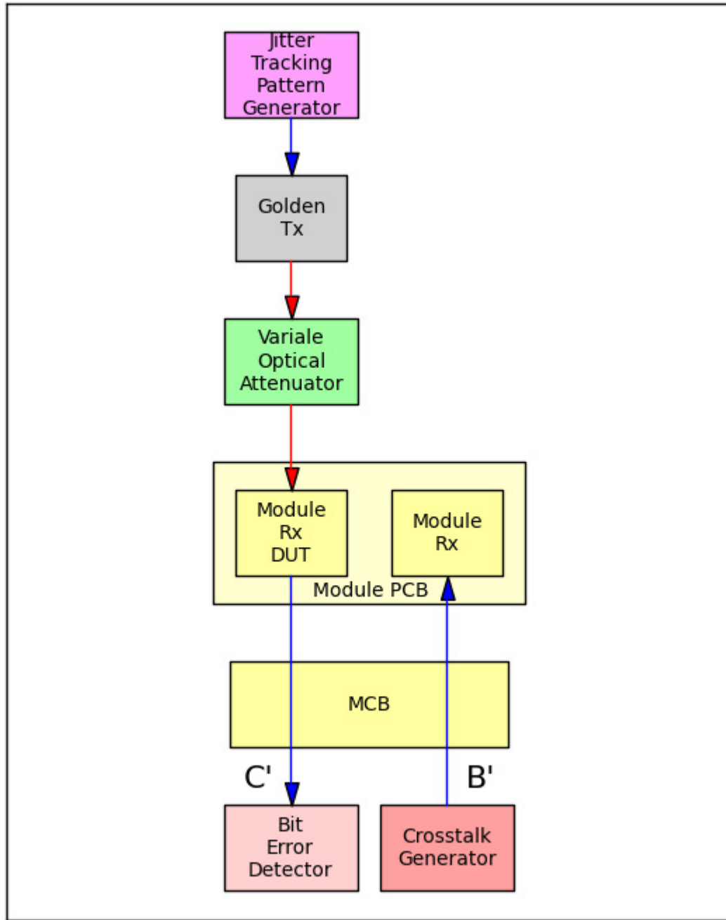
Figure 3.7 - Module optical input jitter tracking test configuration
