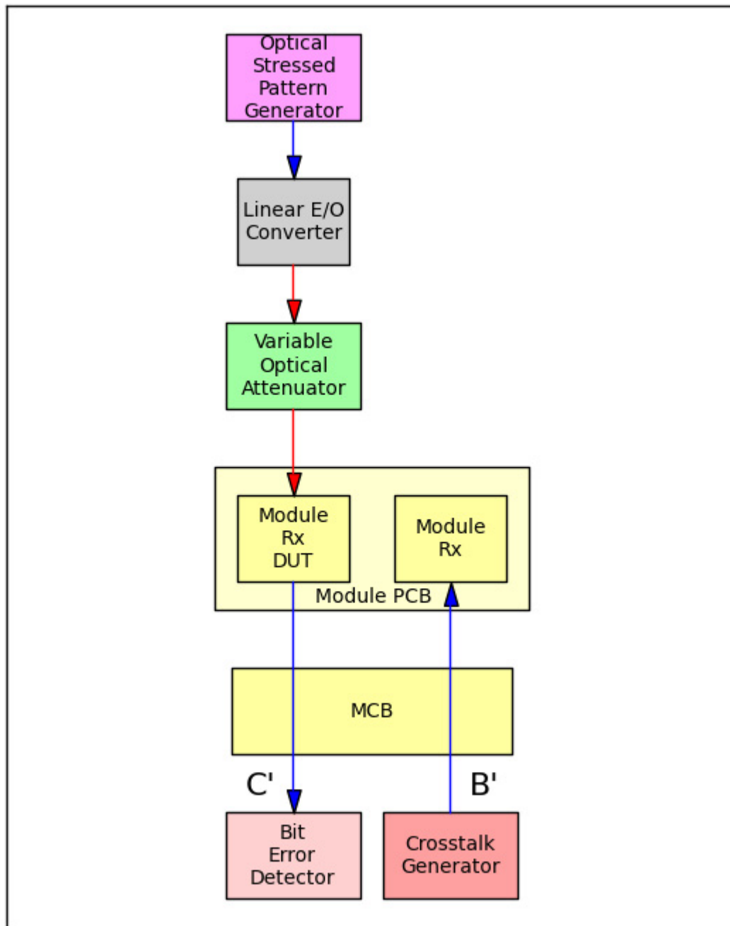
Figure 3.6 - Module optical input stressed receiver sensitivity test configuration
