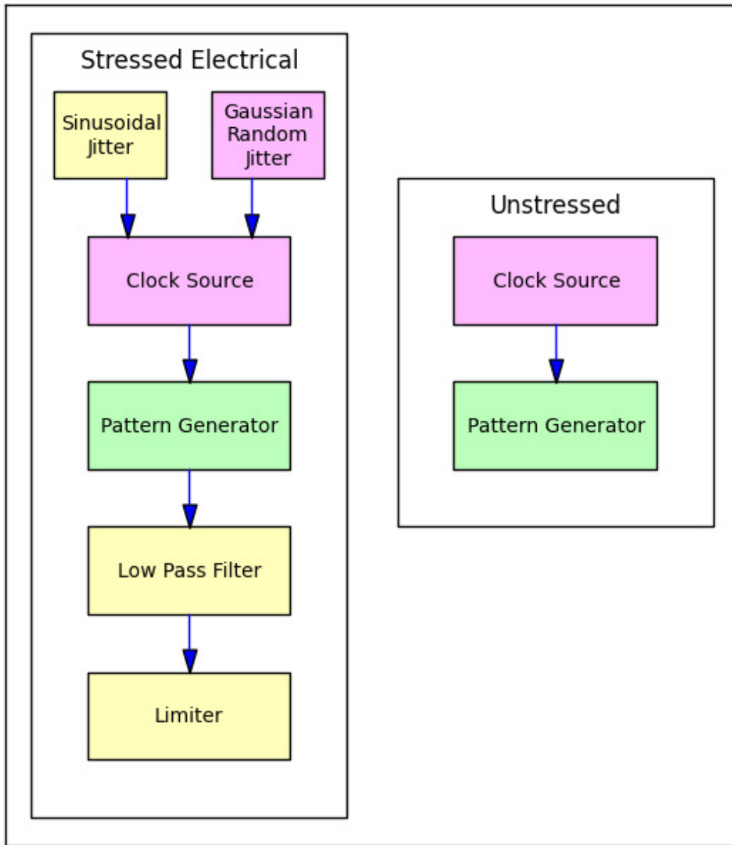
Figure 3.9 - Stressed (left) and unstressed (right) pattern generators
