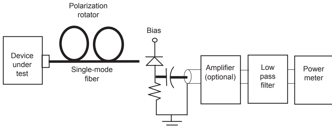
Figure 4.20 - Measurement of laser relative intensity noise ( RIN_{12OMA} ), based on MSQS
