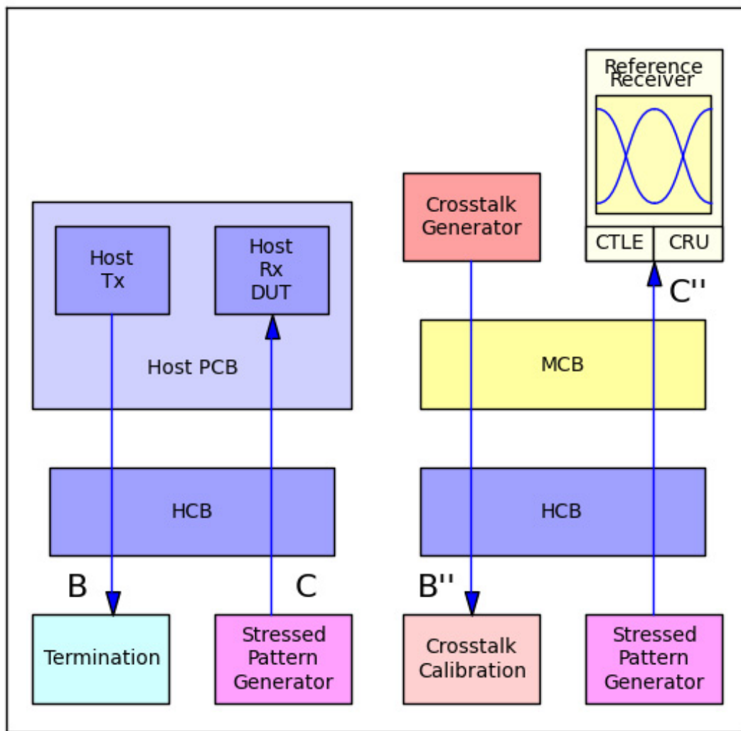
Figure 3.2 - Host input compliance test configuration (left) and calibration (right)
