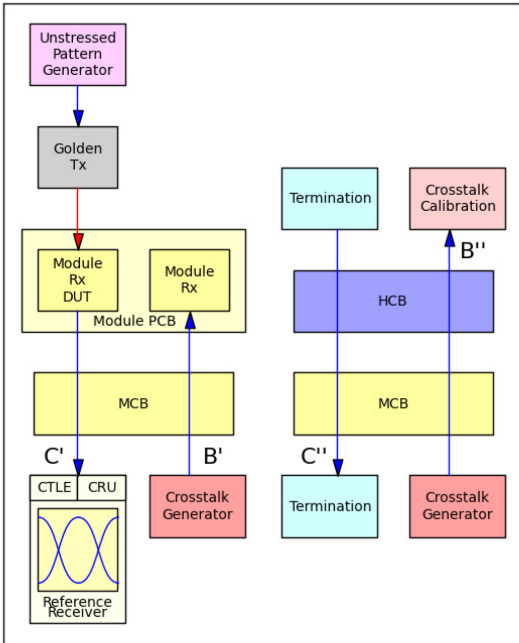
Figure 3.3 - Module electrical output compliance (left) and calibration (right)
