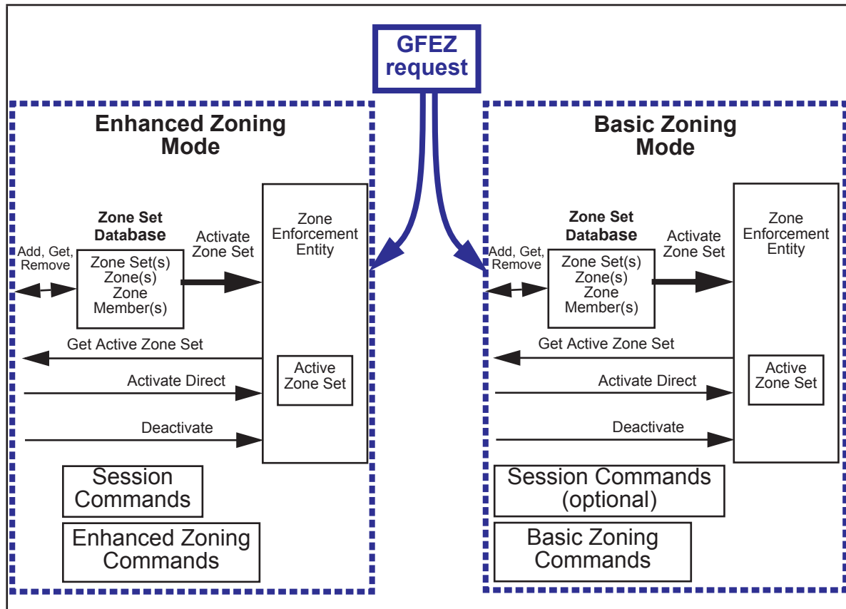
Figure 16 – Zoning Management model
