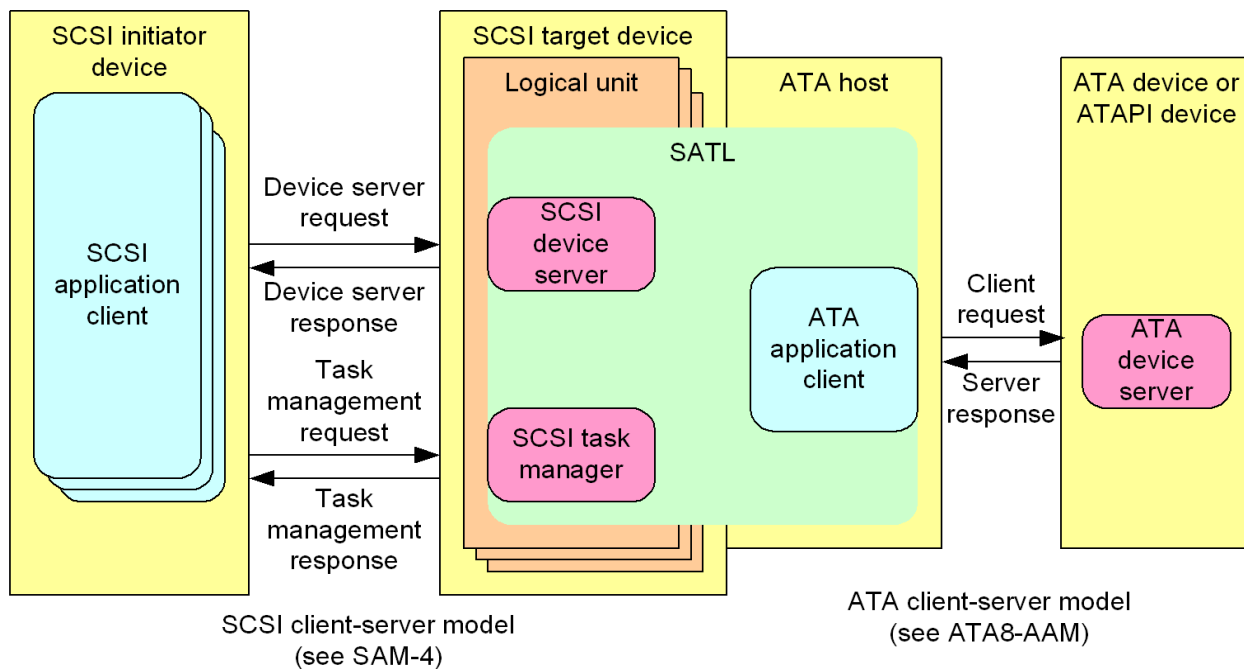
Figure 5 — Example of a SATL between a SCSI application client and an ATA or ATAPI device
