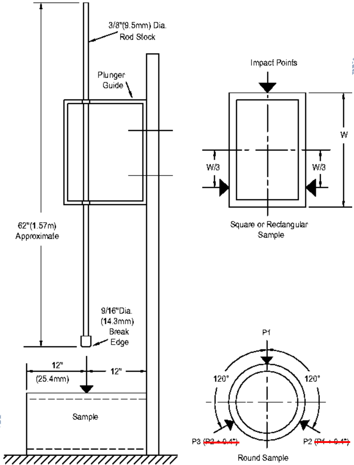
Figure 13.1 Puncture test
