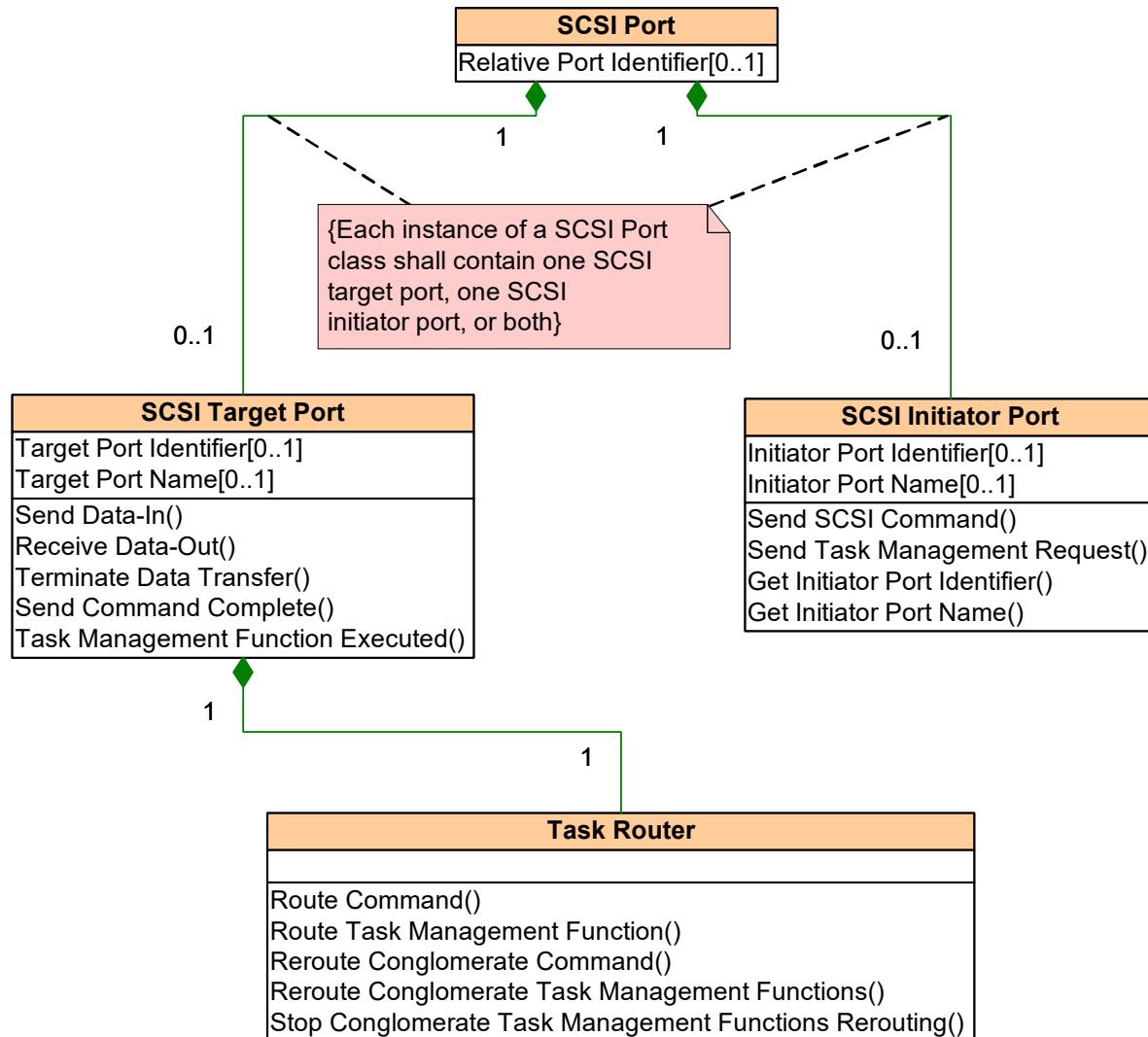
Figure 16 – SCSI Port class diagram
