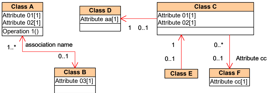
Figure 1 – Examples of association relationships in class diagrams
