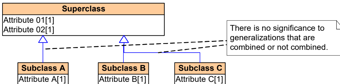
Figure 3 – Example of generalization relationships in class diagrams
