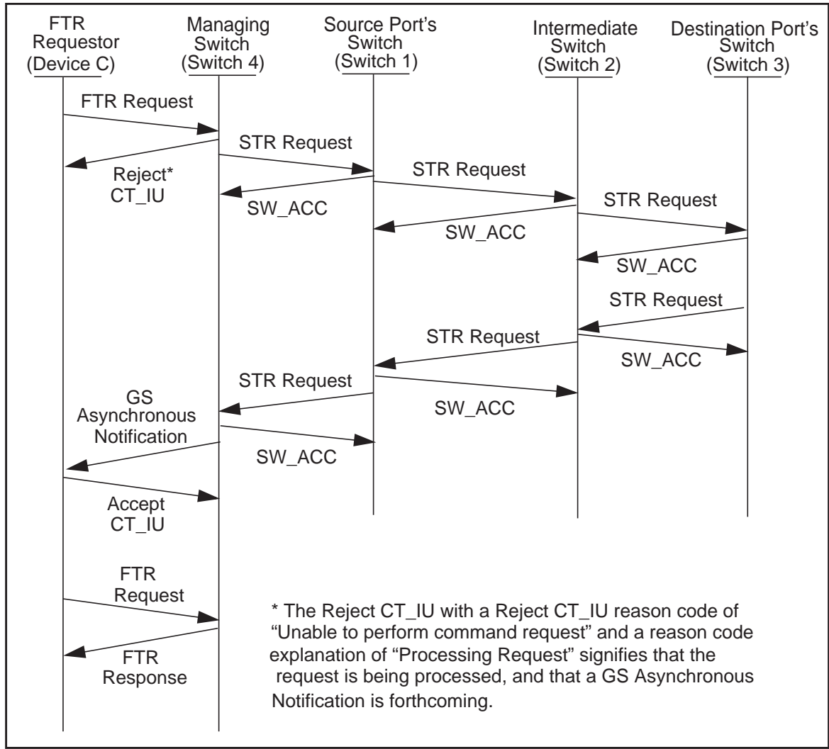
Figure 4 – FTR Processing
